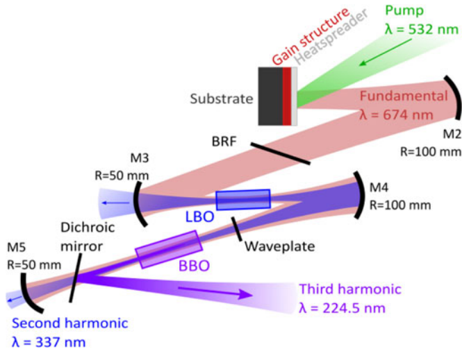
Fig. 1. Schematic diagram of the frequency-tripled SDL. BRF: birefringent filter; M2–M5: high reflectivity mirrors. The heatspreader is a 0.5mm-thick uncoated diamond window.
