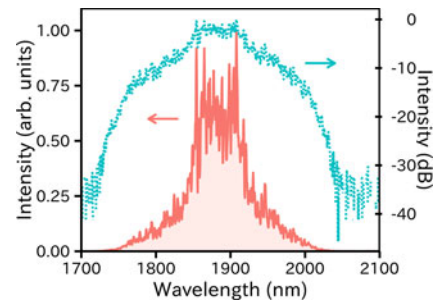
Fig. 5. Optical spectrum measured with a monochromator, plotted in linear scale (red filled curve) and log scale (green dotted curve).
