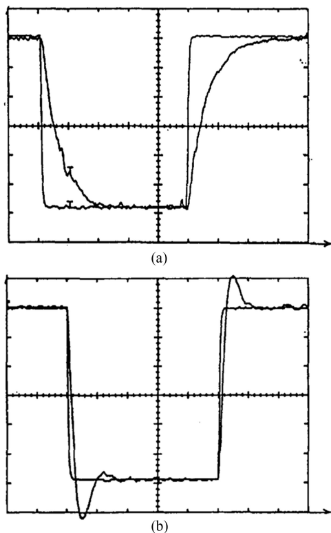
Fig. 5. (a) Sliding mode response to change in inertia (Vertical: 0.2V/div, Horizontal: 1 s/div). (b) PI response to change in inertia (Vertical: 0.2 V/div, Horizontal: 1 s/div).
