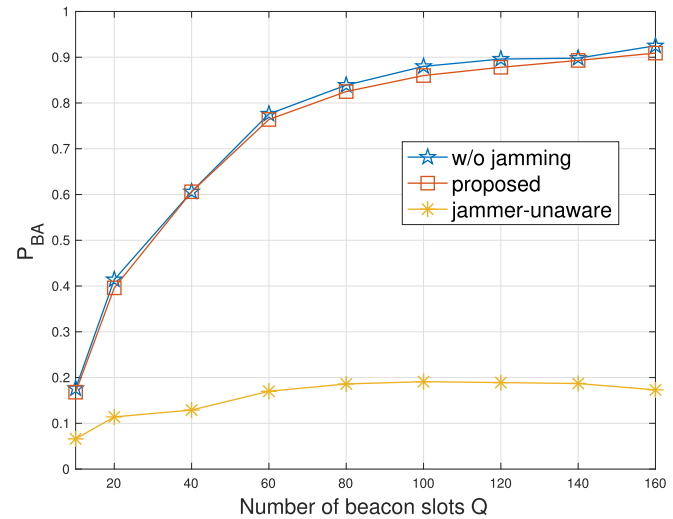
Fig. 7. P_{BA} versus number of beacon slots Q (Case 3, \gamma_B = \gamma_J = 1 , and SJR = -5 dB).
