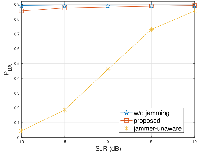
Fig. 10. P_{BA} versus SJR (Case 3, \gamma_B = \gamma_J = 1 , and Q = 100 ).
