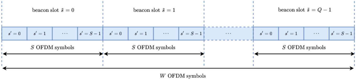
Fig. 2. The BA phase spans a time window of W OFDM symbols, which is divided into Q beacon slots of S OFDM symbols.
