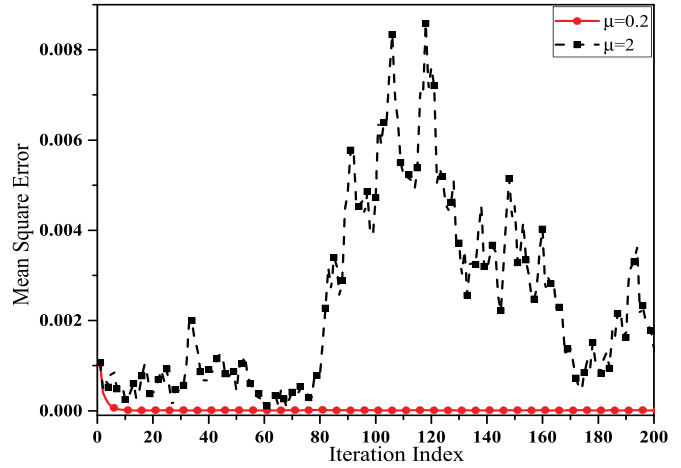
Fig. 9. Convergence and divergence of our intelligent authentication process.
