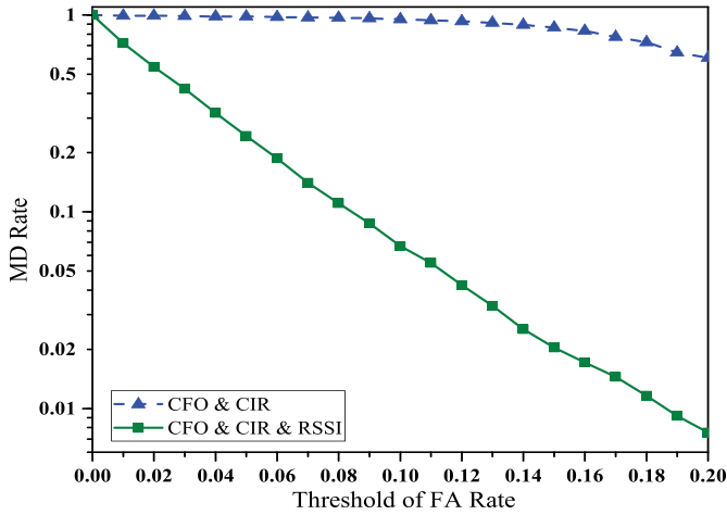
Fig. 7. Authentication performance of our intelligent authentication process relying on the CFO & CIR and CFO & CIR & RSSI scenarios. In this case, Eve can intercept and imitate both the CFO and CIR of Alice.
