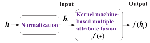
Fig. 3. Kernel machine-based multiple physical layer attribute fusion.
