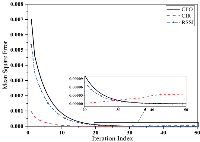
Fig. 4. Training performance of our intelligent authentication process (Algorithm 1) relying on the CFO, CIR and RSSI triplet.
