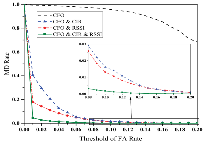
Fig. 6. Authentication performance of our intelligent authentication process relying on the CFO, CFO & CIR, CFO & RSSI, and CFO & CIR & RSSI scenarios. In this case, Eve can intercept and imitate the CFO of Alice.
