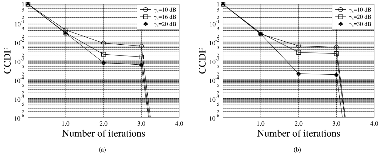
Fig. 6. CCDF of the number of iterations of the GIRCD for the LPIM employing the depth- G interleaver and operating at (a) R_{\mathcal{V}\mathcal{U}} = 1.5 bits/s/ Hz and \gamma_s = 10 dB, 16 dB or 20 dB; (b) R_{\mathcal{V}\mathcal{U}} = 2.5 bits/s/ Hz and \gamma_s = 10 dB, 20 dB or 30 dB. The rate R_{\mathcal{V}\mathcal{U}} is obtained based on (24).
