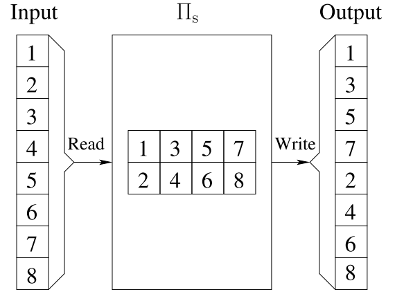
Fig. 2. Illustration of the interleaver \Pi_s with a depth of G = 4 .
