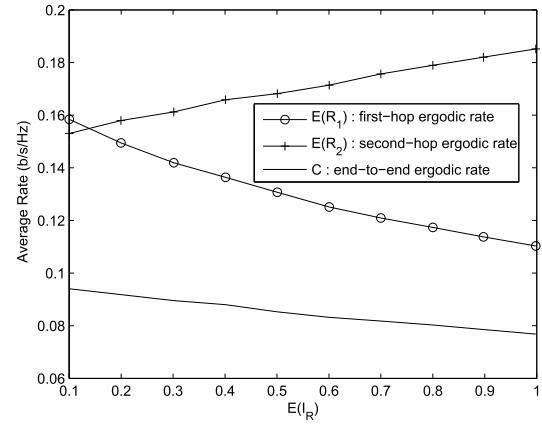
Fig. 11. Average rates (first hop, second hop and end-to-end) versus average interference at the relay \mathbb{E}(I_R) , with \tau = 0.4 , Q_t = 1 dB and varying \mu .
