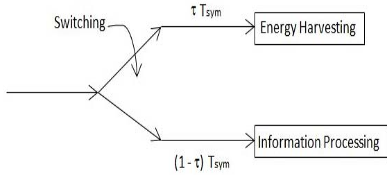
Fig. 2. Time-switching protocol for harvesting energy and information processing.
