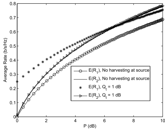
Fig. 5. Average rates at the first and second hops ( \mathbb{E}(R_1), \mathbb{E}(R_2) ) versus P with \eta = 0.3 .
