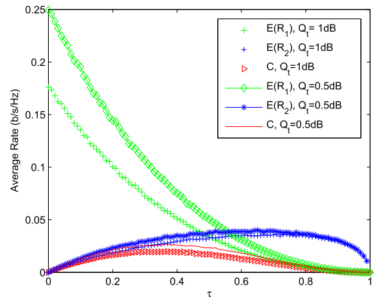
Fig. 7. Average rates at the first and second hops, ( \mathbb{E}(R_1), \mathbb{E}(R_2) ), versus \tau , with \eta = 0.3 and various values of Q_t .
