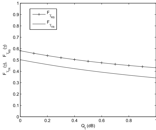
Fig. 6. F_{\gamma_{TR}}(\gamma) and F_{\gamma_{RS}}(\gamma) versus Q_t at \gamma = 0.2 with \eta = 0.3 and P = 1 dB.
