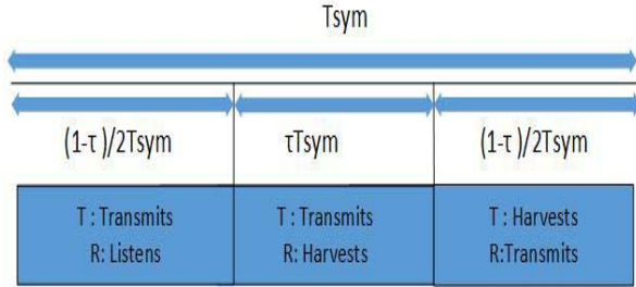
Fig. 3. Illustration of key parameters in time-switching protocol for harvesting energy and information processing.
