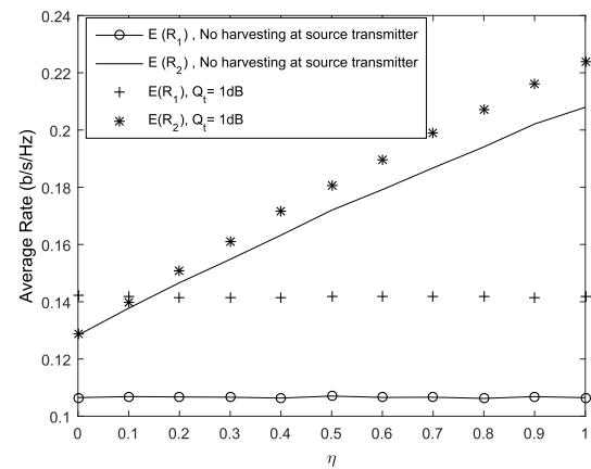
Fig. 8. Average rates (first-hop and second-hop) versus the energy conversion coefficient \eta , with P = 1 dB and various values of Q_t .
