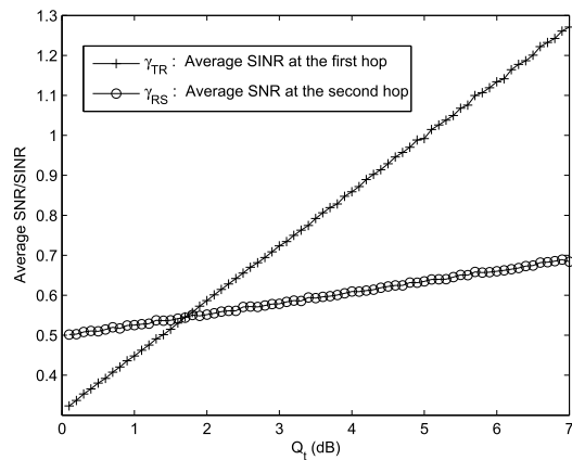
Fig. 10. Average SNR/SINR versus Q_t at \eta = 0.3 with P = 1 dB.
