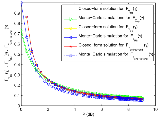
Fig. 4. The CDF of \gamma_{\text{TR}} (first-hop), CDF of \gamma_{\text{RS}} (second-hop), and the CDF of \gamma_{\text{end-to-end}} (end-to-end SNR) versus the power consumed from the fixed batteries P , when \gamma = 0.2 , \eta = 0.3 , K_R = 0.5 and K_S = 0.3 and Q_t = 1 dB.
