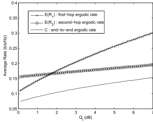
Fig. 9. Average rates (first hop, second hop and end-to-end) versus Q_t at \eta = 0.3 with P = 1 dB.
