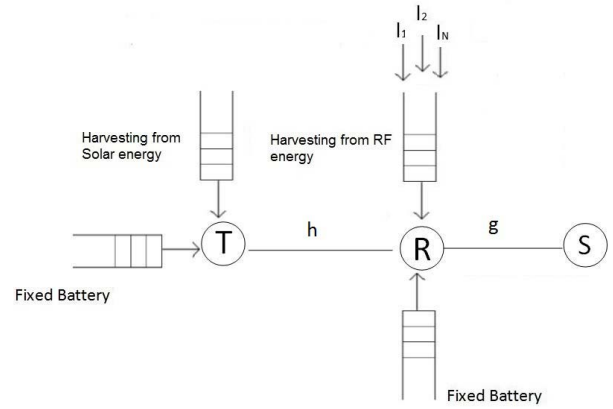
Fig. 1. Relaying system with fixed and energy-harvesting batteries.
