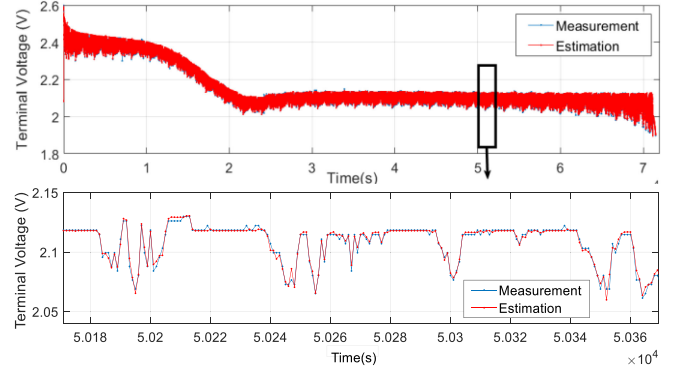
Fig. 5. Terminal voltage validation of Li-S cell model.
