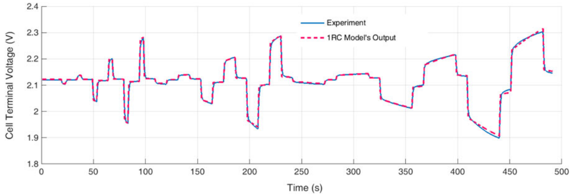
Fig. 7. Li-S cell's terminal voltage prediction using 1RC model.
