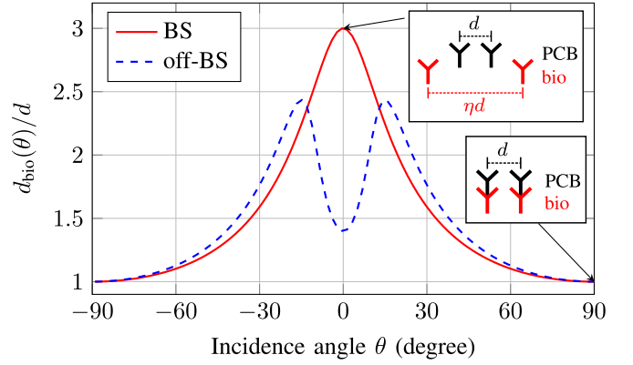
Fig. 2. Angle-dependent, effective biomimetic antenna distance d_{\text{bio}}(\theta) relative to the physical antenna spacing (here: d = \lambda/2 ). The BMAA parameters are identical to the ones in Fig. 1. The insets demonstrate what antenna spacing the biomimetically coupled antennas seem to have (red antennas) compared to the antenna spacing on the PCB (black antennas) for the BS BMAA.
