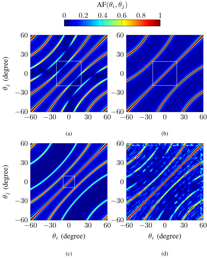
Fig. 5. (a) AF for a MIMO BMAA according to Layout A in Fig. 4 and Table III (AFR = -19.3^\circ, \dots, 19.3^\circ ). (b) AF of an array with the same aperture as Layout A in BS direction (AFR = -18.8^\circ, \dots, 18.8^\circ ). (c) Corresponds to the AF of the physical aperture on the PCB without BMCs (AFR = -9^\circ, \dots, 9^\circ ). The rectangles indicate the AFRs of the configurations. (d) Shows the measurement of (a) presented in Section V.
