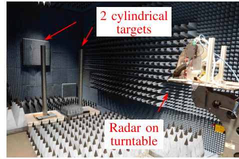
Fig. 11. Two cylindrical targets with identical RCS are arranged symmetrically to the \theta = 0^\circ BS direction of a turntable. The measuring radar is mounted on the turntable.
