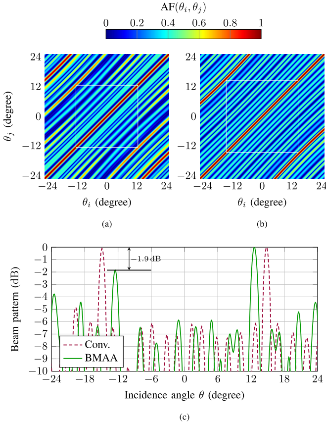
Fig. 8. AFs of the example “Genetic Array 2” for the genetic optimization (a) with and (b) without BMCs and (c) their BP at the angle \theta_0 where their first grating lobe occurs (conventional array \theta_0 = 14.8^\circ , BMAA \theta_0 = 12.6^\circ ).
