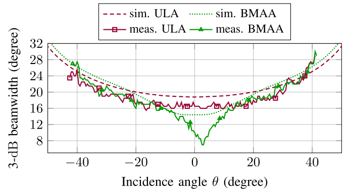
Fig. 12. Simulated and measured 3-dB BW for the deterministic MIMO BMAA with smaller BW of Table III and the identical antenna board without BMCs, corresponding to the AFs in Fig. 6.
