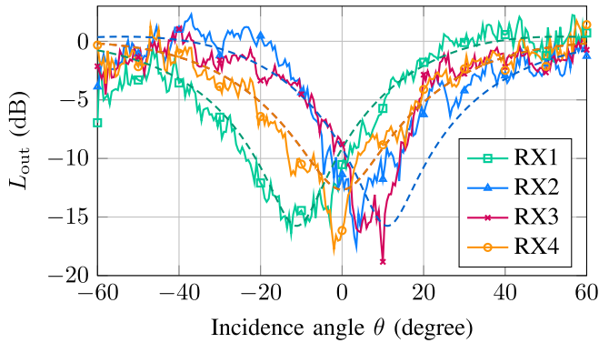
Fig. 10. Measurement (solid lines) and theoretical curves (dashed lines) of L_{out} for the deterministic array with smaller BW according to Layout B of Fig. 4 and the values of Table III for transmitter TX1. RX1 and RX2 form the off-BS BMAA ( \eta = 1.4 , \zeta = 2.5 ) and RX3 and RX4 the BS BMAA ( \eta = 4.3 , \zeta = 0 , theoretical curves overlapping).
