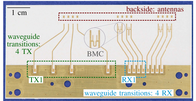
Fig. 9. Antenna board for the deterministic MIMO BMAA with smaller BW of Table III: the patch antennas are located on the backside of the displayed PCB. As there are several RX antennas on this PCB, we marked the waveguide transitions of the respective four RX antennas.
