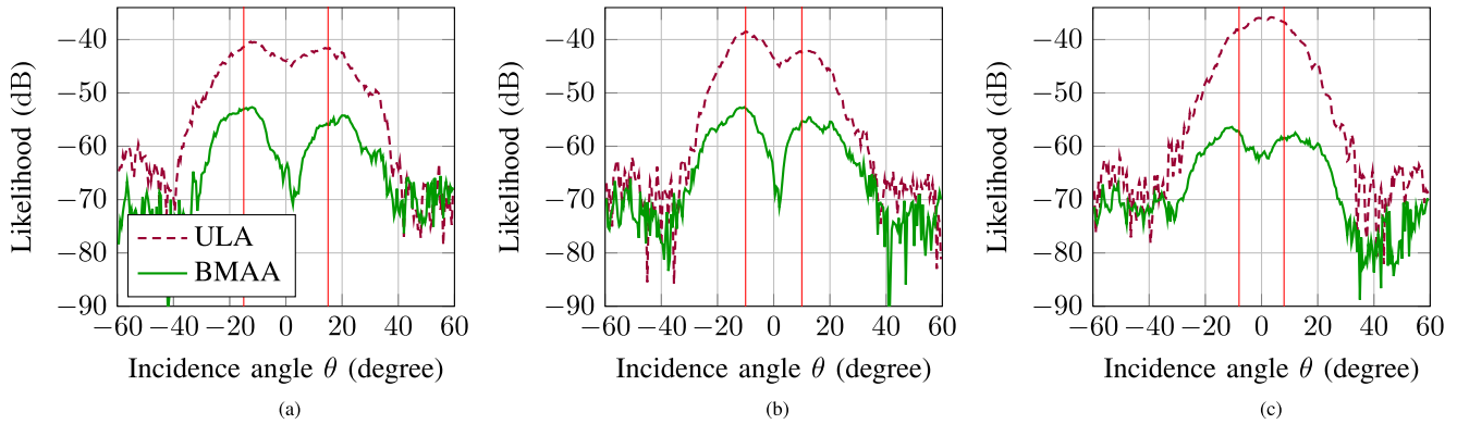
Fig. 13. Measured, un-normalized likelihood for two targets in the same range-velocity bin for the deterministic MIMO BMAA with smaller BW of Table III (—) and the identical array without BMCs but the same antenna positions (----). The targets are positioned symmetrically around BS and their true DOA is indicated with red lines. (a) 2 targets at \pm 15^\circ . (b) 2 targets at \pm 10^\circ . (c) 2 targets at \pm 8^\circ .
