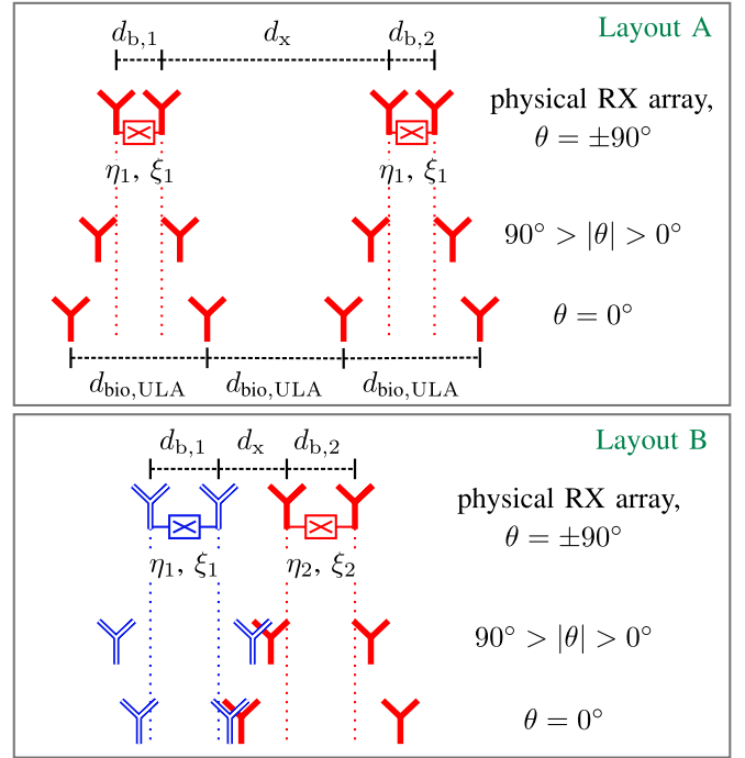
Fig. 4. Two exemplary layouts of four-element RX arrays utilizing BMAAs as part of the array. The effective biomimetic aperture is identical to the physical aperture on the PCB for \theta = \pm 90^\circ for both layouts, because d_{b,1} = d_{b,2} = \lambda/2 is chosen here. Below the physical RX array, it can be seen how d_{\text{bio}}(\theta) influences the RX aperture. Antennas of BS BMAAs are drawn red filled, antennas of off-BS BMAAs blue striped.
