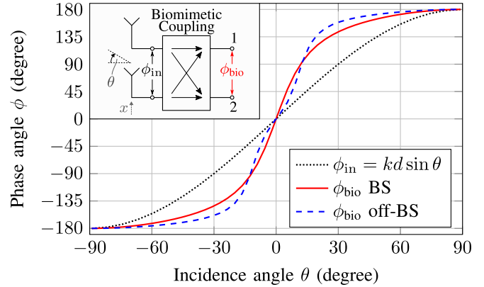
Fig. 1. Biomimetic output phase progression \phi_{\text{bio}} for a BS BMA (—) and an off-BS BMA (---) compared to the conventional phase progression (·····) for the same antenna spacing d = \lambda/2 [13]. The BMA parameters are \eta = 3 , \zeta = 0 (BS) and \eta = 1.4 , \zeta = 2.5 (off-BS).
