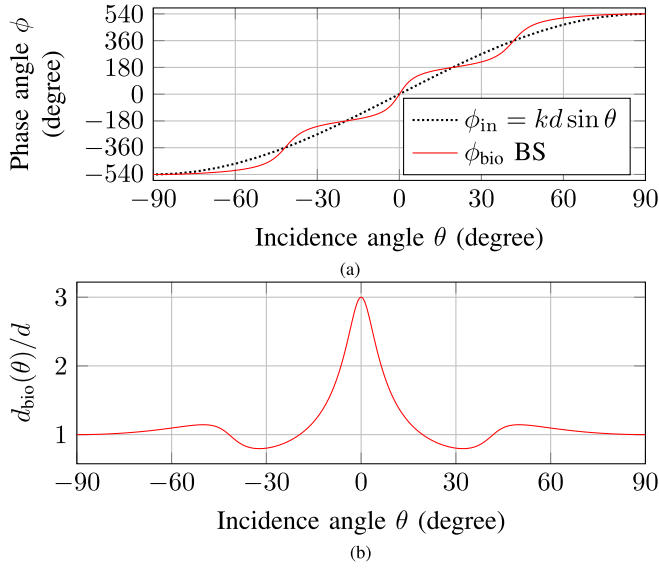
Fig. 3. (a) Exemplary phase progression and (b) normalized effective biomimetic antenna distance d_{\text{bio}}(\theta) for a BS BMAA with physical antenna spacing d > \lambda/2 . Specific parameters: \eta = 3 , \xi = 0 , and d = 1.5\lambda .
