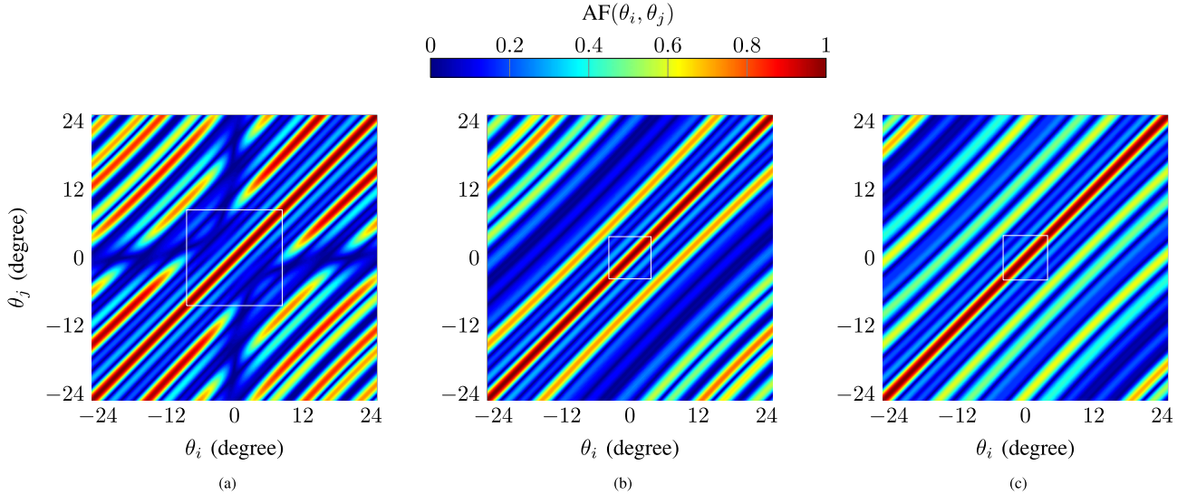
Fig. 7. AFs for the example “Genetic Array 1”: (a) optimized array configuration including BMCs in the RX array, (b) same array configuration without BMCs, and (c) independently optimized array without biomimetic coupling applied. Using the same PCB and antenna restrictions, the optimization including BMCs in (a) could yield a much larger AFR (marked by the square) compared to the optimization in (c).
