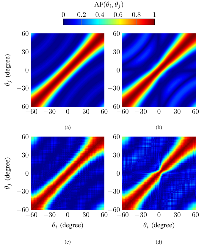
Fig. 6. (a) Simulated and (c) measured (see Section V) AF of the virtual array build up by two four-element ULAs (TX and RX) with an antenna spacing of d = (\lambda/2) . The AF for the same antenna placement utilizing BMAs in the RX array corresponding to Layout B in Fig. 4 and Table II is shown in (b) through simulation and (d) through measurement. The array parameters are selected identical to the ones of Table III (second column).
