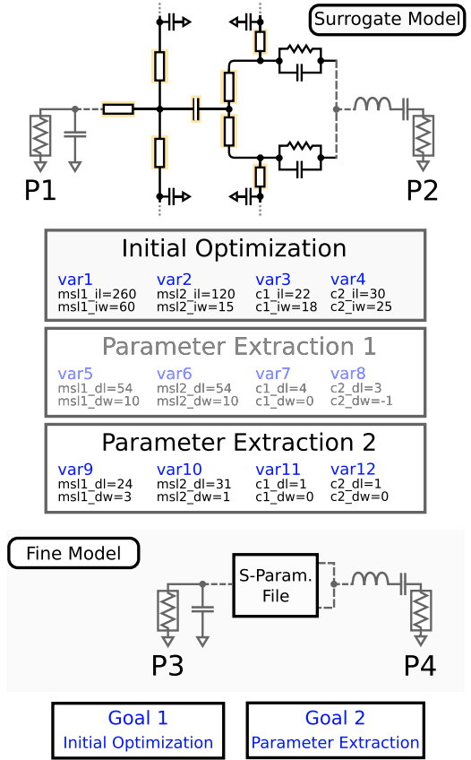
Fig. 8. Illustration of a reference implementation of algorithm C in a schematic editor such as Keysight ADS. The relevant elements of the surrogate model (top) are parameterized using the variable blocks below. Each parameter extraction variable block pertains to one iteration of the algorithm.
