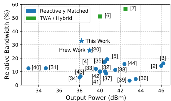
Fig. 16. Relative 1-dB bandwidth over maximum output power of recent GaN HPA publications.
