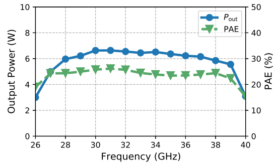
Fig. 15. Output power and PAE in 3-dB gain compression in the Ka-band frequency range. The MMIC was biased at a drain voltage of V_D = 15\text{ V} and a drain current density of i_D = 50\text{ mA/mm} .
