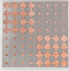
Fig. 20. Photograph of the prototyped checkerboard metasurface.
