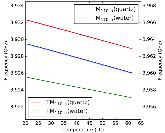
Fig. 6. TM_{110} measured frequency versus temperature with measurement modes on the left axis and reference modes on the right axis.
