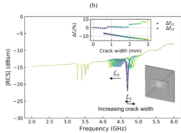
Fig. 7. Simulated RCS spectra of the chipless RFID sensor tag showing resonant frequency shift for different crack orientations and widths. (a) Horizontal crack. (b) Vertical crack. (c) Diagonal crack.
