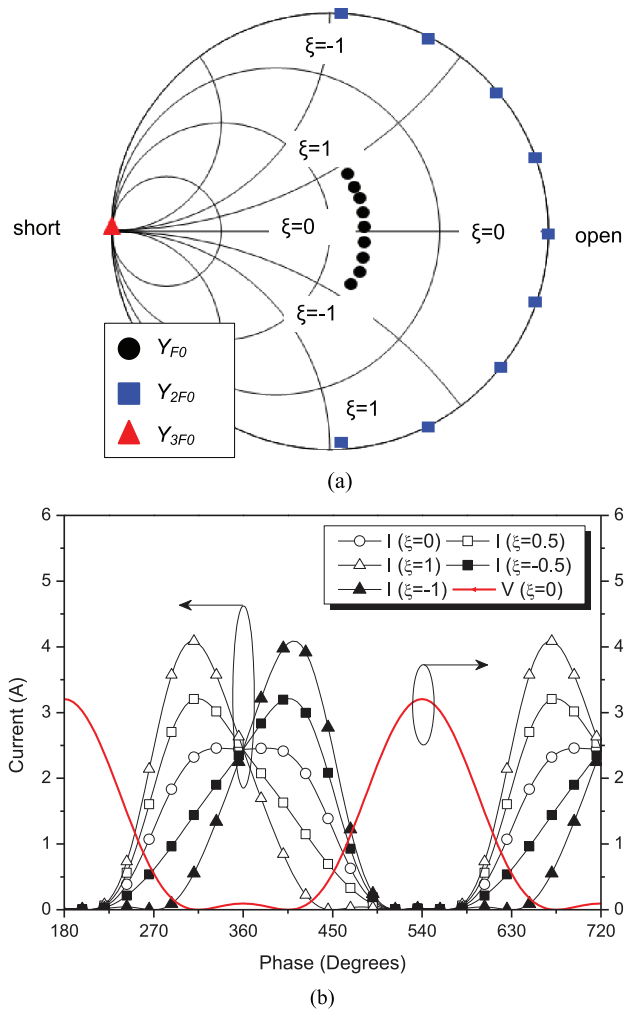
Fig. 4. (a) Ideal contours of continuous class- F^{-1} loading conditions. (b) Ideal contours class- F^{-1} resulting waveform combinations.
