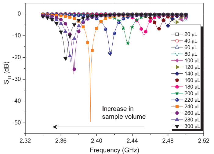
Fig. 3. Measured \text{TM}_{010} -mode circular cavity response showing resonant shift due to varying water volume.
