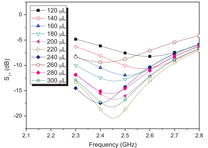
Fig. 8. S_{11} of the integrated TM_{010} -mode circular cavity resonator for varying sample volumes.
