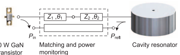
Fig. 9. Output matching network and incident and reflected power monitoring by quarter-wave directional coupler.
