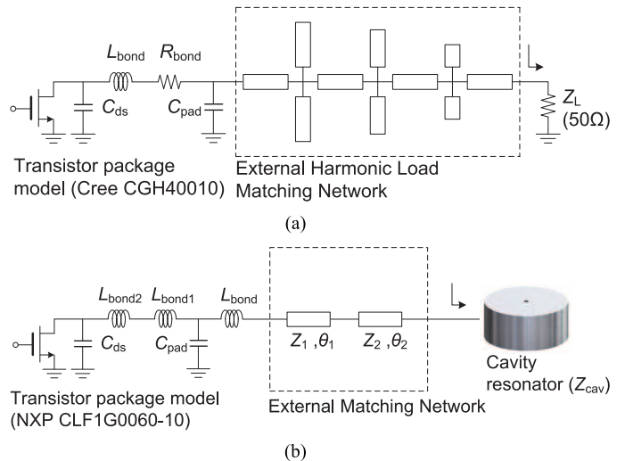
Fig. 1. Matching circuit design incorporating package parasitic components for (a) conventional 50- \Omega continuous class- F^{-1} design using a CREE 10-W GaN (CGH40010) power transistor [7]. (b) Simplified, compact direct match design, again incorporating package parasitics, using a similar NXP 10-W GaN device (CLF1G0060-10).
