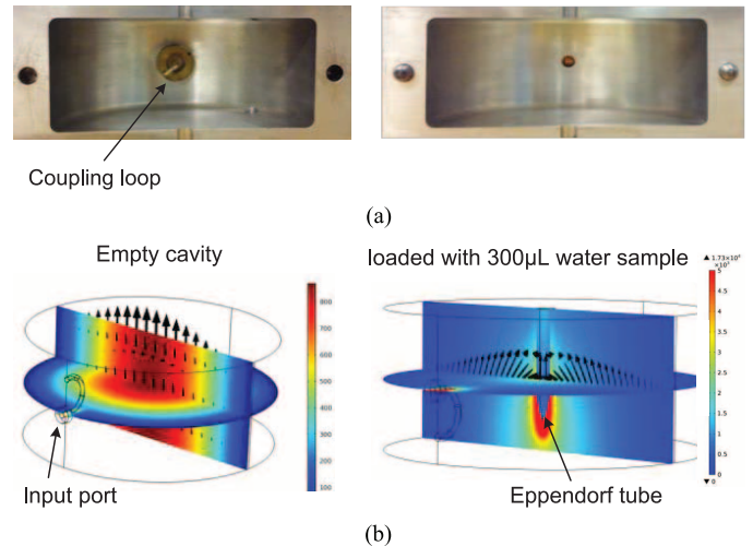
Fig. 2. (a) \text{TM}_{010} circular cavity showing both hemispheres as well as the coupling loop. (b) E -field distribution (V/m)—simulated using COMSOL multiphysics package at 2.5 GHz.
