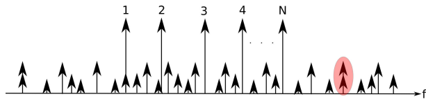
Fig. 1. Multicarrier scenario in which two different PIM tones fall at the same frequency.
