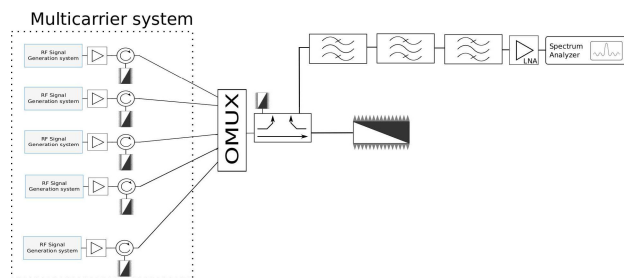
Fig. 2. Schematic of the PIM measurement setup based on the multicarrier facility, able to combine up to five high-power carriers at once.
