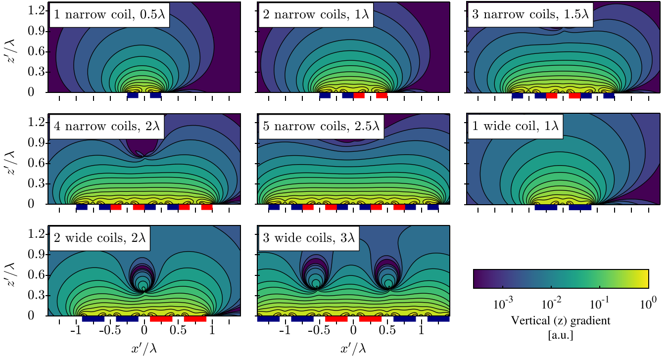
Fig. 4. Logarithm of the magnitude of the vertical ( z ) magnetic field gradient, \log |\nabla_z H| , above the surface of the sets of coils. Like Fig. 3, the plots show the x'z' -cross section at the y -symmetry plane. The coils are indicated in red and blue. The magnetic field gradient is normalized with its maximum value encountered across all considered configurations. The asymmetry in the x' -coordinate is due to the \alpha = 12^\circ angle between the z - and z' -axes (see Fig. 1).
