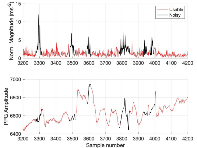
Fig. 4. Example of data showing interference with motion artifacts. Normalized accelerometer signal (above) and red LED signal (below). Black lines illustrate y periods of the interference caused by the movement of artifacts as determined by the masking step.
