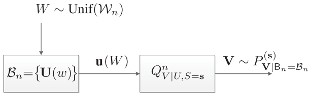
Fig. 1. Coding problem with the goal of making P_{\mathbf{V}|\mathbf{B}_n=B_n}^{(s)} resemble Q_{V|S=s}^n .
