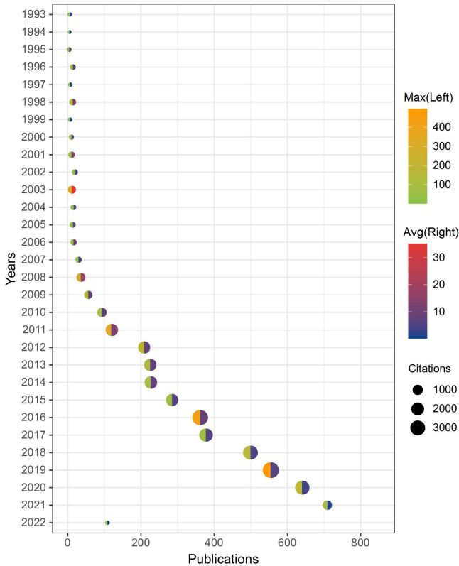
Fig. 3. Publications overview.
