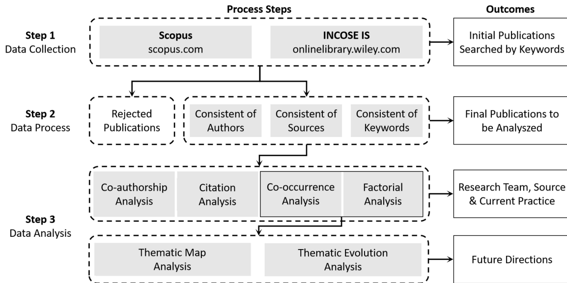
Fig. 2. Research methodology.
