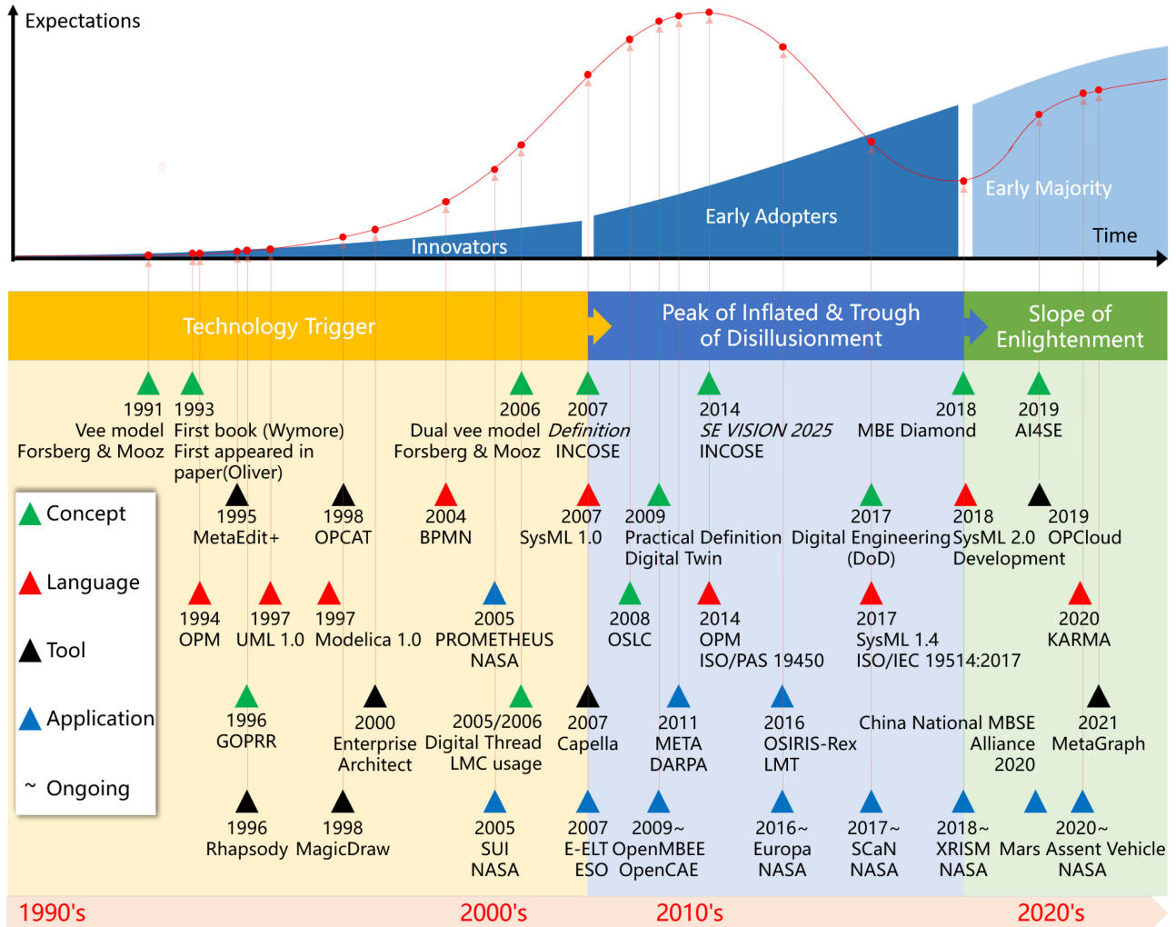
Fig. 1. Timeline of MBSE.
