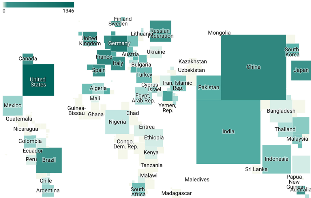
Fig. 6. Researcher distribution.
