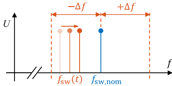
Fig. 1. Principle of spread spectrum.
