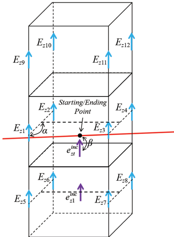
Fig. 5. Interpolation scheme for the electric fields at the starting or ending points of each segment of oblique transmission line.
