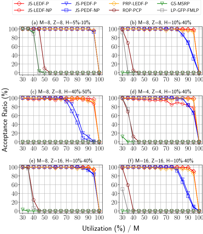
Fig. 2. Schedulability of different approaches for frame-based task sets.
