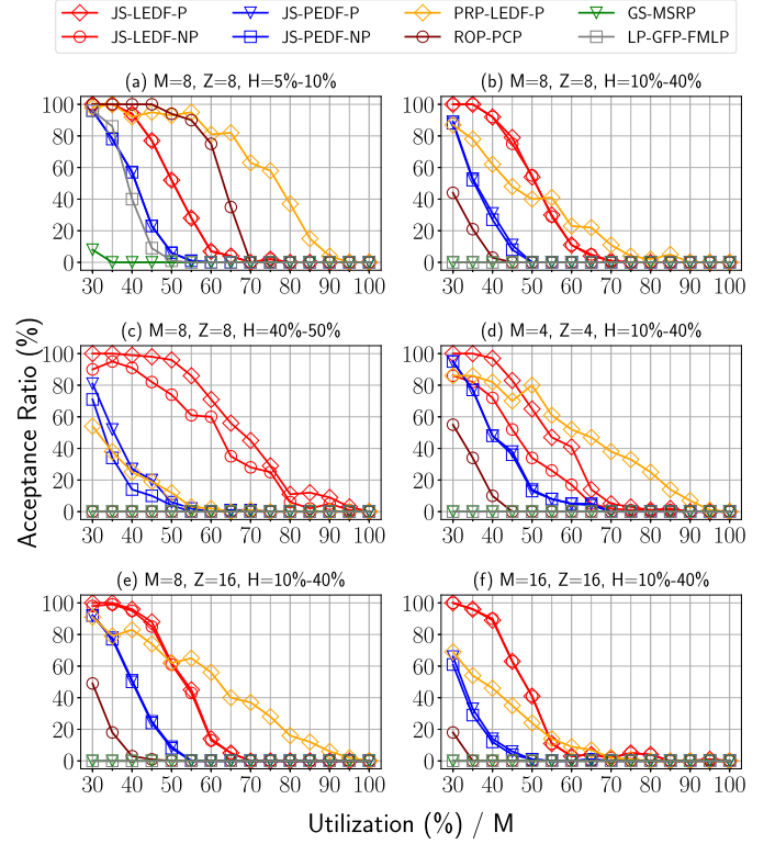
Fig. 3. Schedulability of different approaches for periodic task sets.
