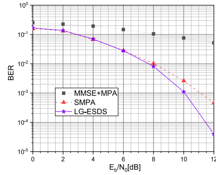
Fig. 10 BER comparison of MMSE+MPA, SMPA and LG-ESDS over the 4 \times 4 MIMO channel.
