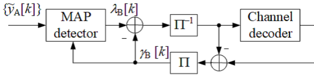
Fig. 8 Schematic of the IDD receiver.
