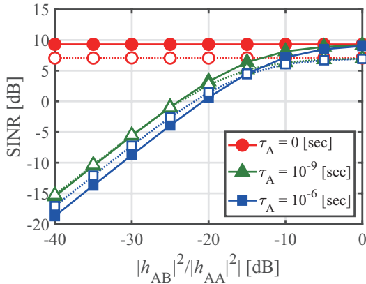
(a) SINR vs. \zeta = |h_{AB}|^2 / |h_{AA}|^2 .
