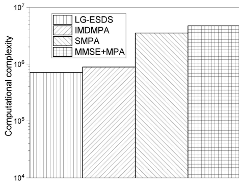
Fig. 11 Computational complexity comparison of MMSE+MPA, SMPA, IMDMPA and LG-ESDS over the 2 \times 2 MIMO channel.
