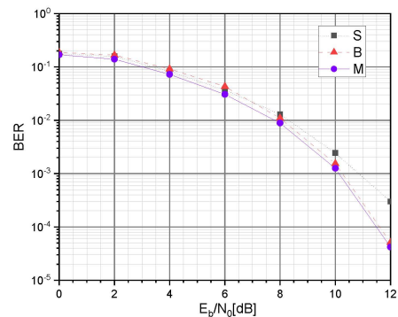
Fig. 5 Find the optimal E_b/N_0 value for the training of LG-ESDS over the 2×2 MIMO channel.
