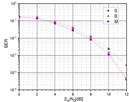
Fig. 6 Find the optimal E_b/N_0 value for the training of LG-ESDS over the 4×4 MIMO channel.
