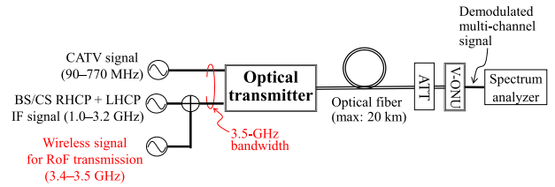
Fig. 3 Proposed configuration in this study.
