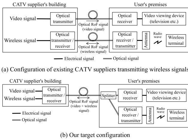
Fig. 1 Equipment and network for transmitting video and wireless signals.
