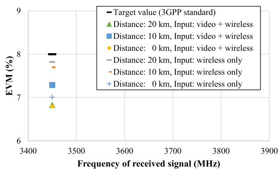
Fig. 8 Quality of received signal (wireless signal band).
