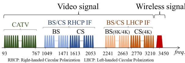
Fig. 4 Overview of frequency spectrum of the input signal.
