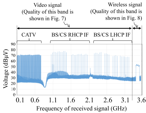
Fig. 6 Raw waveform of received signal.
