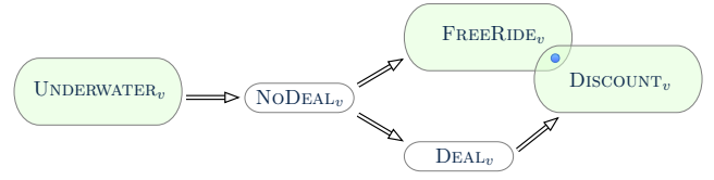
Fig. 2. The structure of a preference poset of a party v in an h-swap system. The arrows symbolize the preference relation. The one outcome in \text{DISCOUNT}_v \cap \text{FREERIDE}_v is \langle A_v^{in} \mid \emptyset \rangle .
