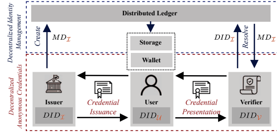
Figure 2: Overview of the Decentralized Identity Model. Each entity is identified by a pseudonymous DID . The issuer \mathcal{I} issues a credential to the user \mathcal{U} . Upon presentation of the credential, the verifier \mathcal{V} can verify its validity without interacting with \mathcal{I} by resolving the issuer DID to obtain the issuer metadata MD_{\mathcal{I}} .
