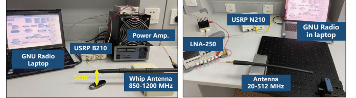
Fig. 10. The experimental setup for DeHiREC is composed of two categories. (1) EMR receiver (right) . We adopt a whip antenna to capture the weak EMR signals, connecting to a low noise amplifier to filter noise and amplify the signal. The EMR signal is then transmitted to the laptop by USRP and then adopt signal analysis. (2) EMI transmitter (left) . We modulate the baseline signal and carrier by USRP and amplify the EMI signal by the power amplifier. The generated EMI signal is emitted by a whip antenna.
