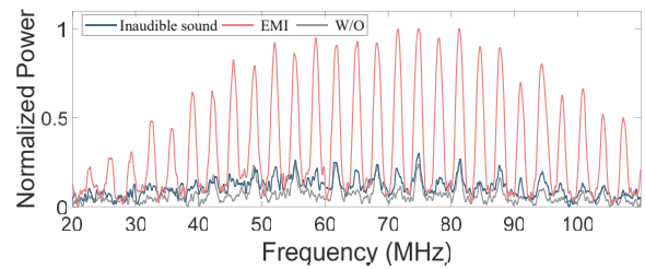
Fig. 6. The power spectrum of the EMRs under two stimulations. Results show that electromagnetic interference can significantly increase the intensity of EMR, yet inaudible sound injection presents poor performance.
