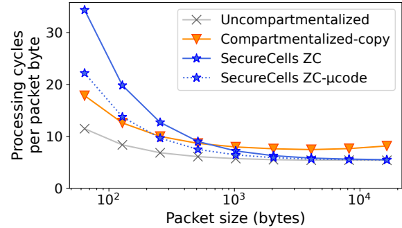
Figure 7. Packet processing cycles-per-byte comparison.
