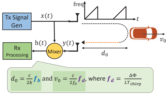
(a) Radar signal processing
