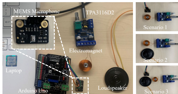
Fig. 4. The setup of Experiment I and three experimental scenarios where a separate microphone, a separate loudspeaker, and a combination of the two in a varying magnetic field.
