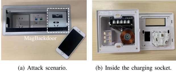
Fig. 19. MagBackdoor in a charging socket.
