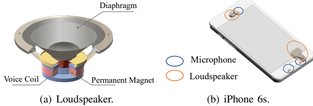
Fig. 2. An illustration of the structure of loudspeakers and the distribution of loudspeakers and microphones in smartphones.
