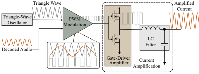
Fig. 10. The signal processing flow of Power Amplification.
