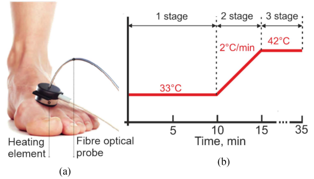
Fig. 5. (a) Location of the fibre optical probe on the volunteer's foot. (b) Study protocol with the heat test.
