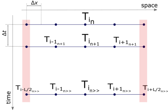
Fig. 1. The 1D object is modeled as a grid of L-nodes. The central node i represents the target lesion, directly treated by the laser beam. Over time, the temperature increases along the grid progressively affecting all the nodes. Boundary conditions are applied at the extremities (red).
