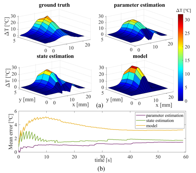
Fig. 10. Temperature prediction via state and joint Bayesian estimation for agar-gel phantom in 2D configuration, using 3 observations in (0,-3), (2,4), (0,1). (a) Temperature distribution at 55 s of the heating process. (b) Time evolution of the mean temperature error for the model (yellow line), state (green line) and parameter (purple line) estimation with respect to the ground truth.
