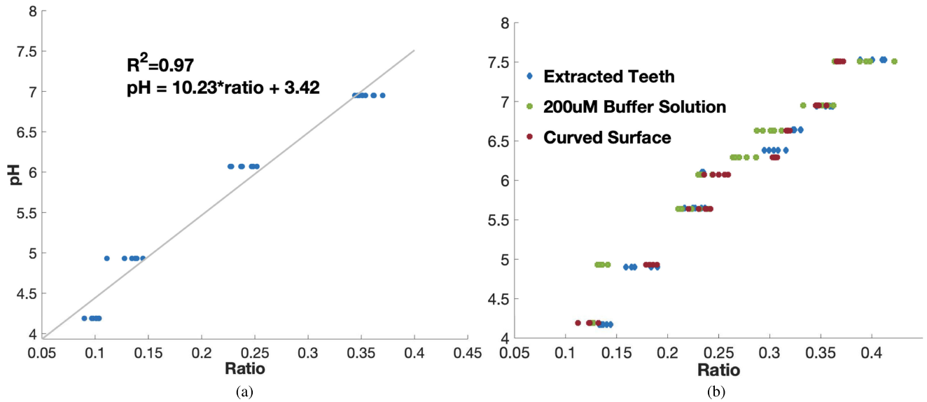
Fig. 4. (a) Calibration curve using buffer solution in a 1 mm cuvette. Ratio is given by 1. (b) Verification of calibration curve using 200 \mu\text{M} buffered fluorescein in 1 mm cuvette, on extracted human teeth, and on artificial curved teeth surfaces (occlusal, interproximal, and buccal surfaces of artificial teeth). A drop of fluorescein is added on different teeth surfaces and pH is measured using O-pH.
