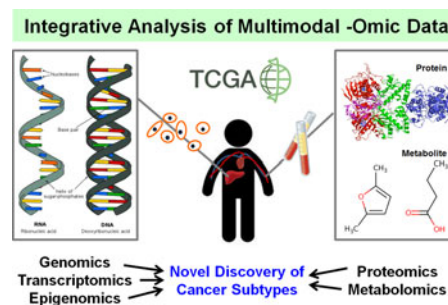
Fig. 2. Integrative analysis of multi-omic data leads to the improved understanding of cancer mechanisms, which in turn enables more precise classification of cancer subtypes.
