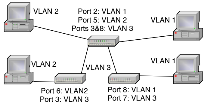
Fig. 10. VLAN segmentation.
