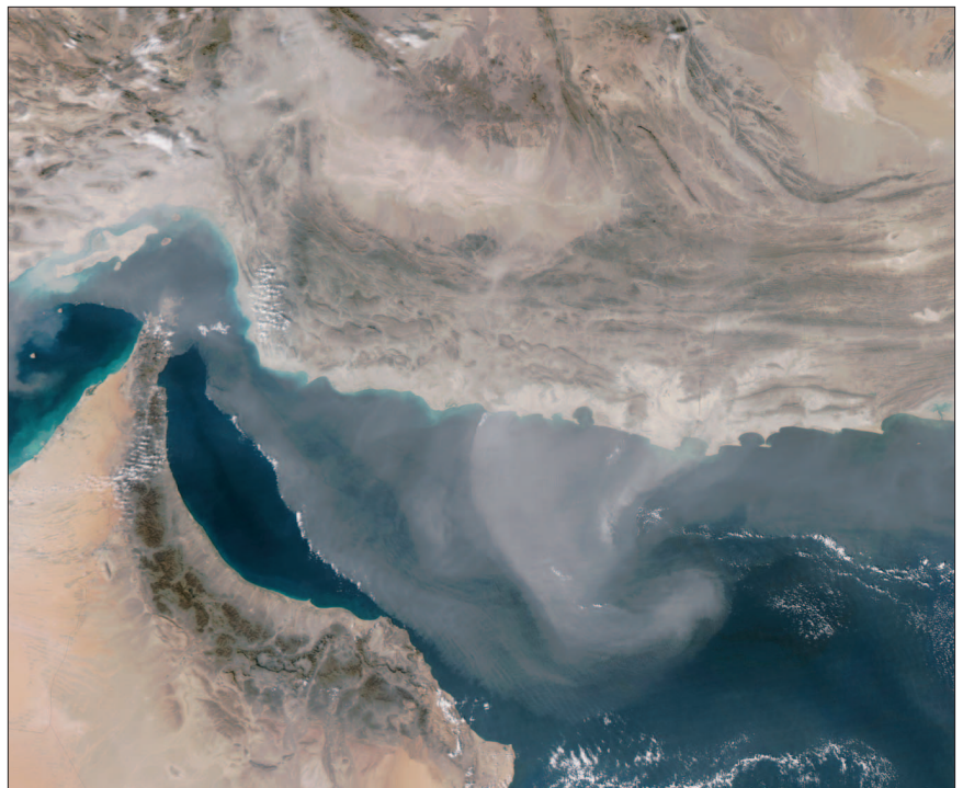
Figure 4. Dust storm in the Persian Gulf as captured by MODIS in November 2003.
