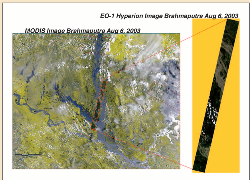
Figure D. Examples of low-resolution MODIS imagery (left) and high-resolution EO-1 imagery (right) from the Flood Sensorweb capturing Brahmaputra River flooding in India, August 2003.
