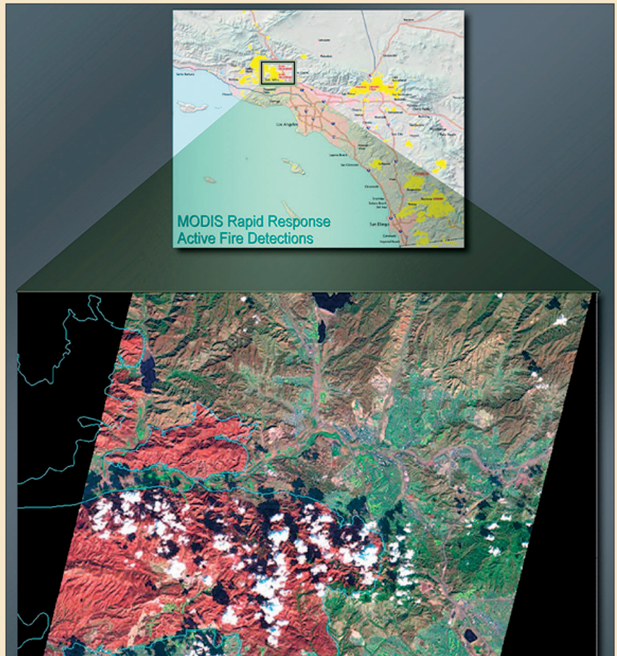
Figure B. Sensorweb trigger images for the October 2003 Southern California fires. Above is the MODIS Active Fire Map display. Below is the EO-1 Hyperion image acquired via sensorweb trigger of the Simi/Val Verde fire area used in Burned Area Emergency Reclamation.
