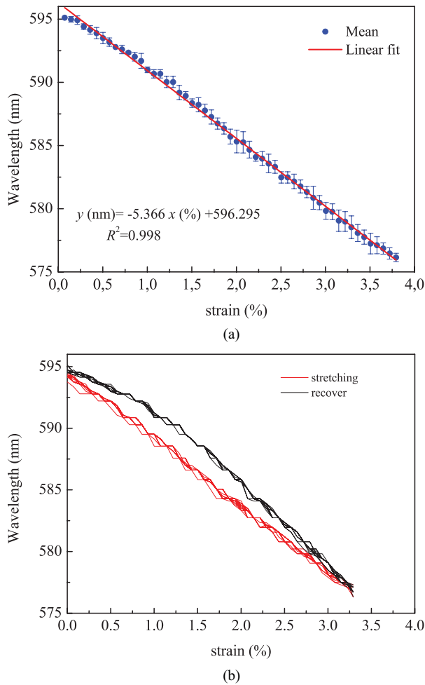
Fig. 5. Typical experimental results obtained in the first scenario. In both cases, the relationship between strain and the wavelength of the loss feature is shown. (a) Typical response of the sensor to the ramp-like loading of the LPG mPOF. Step size: 37.5 \mu\text{m} (0.07). (b) Typical response of the sensor to the ramp-like cyclical loading of the LPG mPOF. Number of repetitions: 15. Step size: 37.5 \mu\text{m} (0.07).
