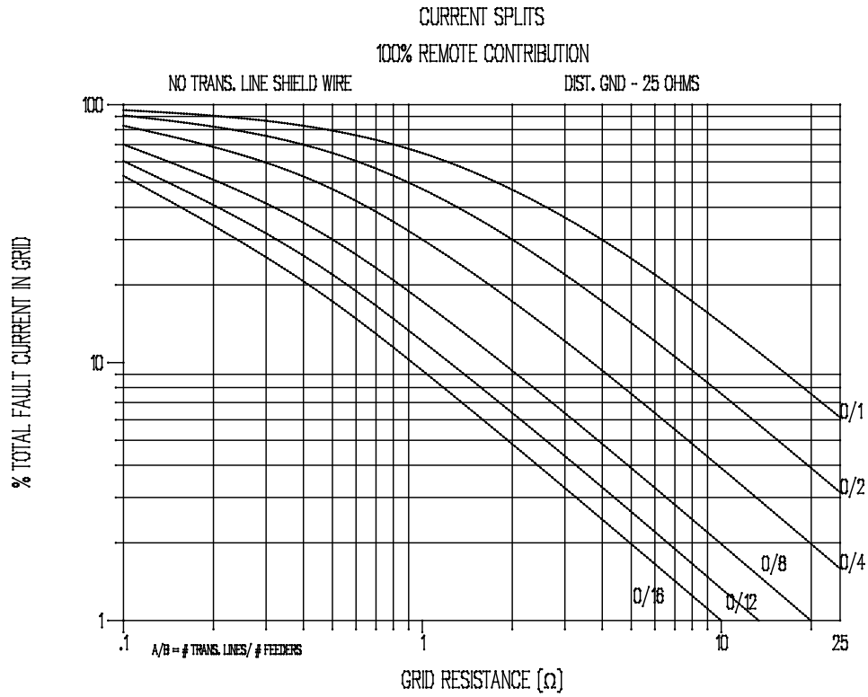
Figure C.15—Curves to approximate split factor S_f
