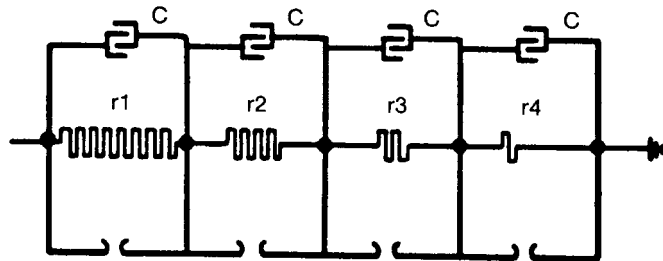
Figure 17—Soil model
