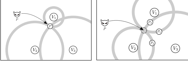
Figure 14. Location Verification and Location Hijacking: P hijacks the location of P' , for example by hijacking the distance bounding protocol instances of P' with respect to the verifiers.
