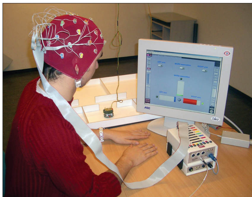
Fig. 2. Noninvasive BMI based on the analysis of EEG signals, i.e., the brain electrical activity recorded from electrodes placed on the scalp (colored spots in the red cap worn by the person). The user is mentally driving a mobile robot between rooms in a house-like environment, making it turn or move forward. Alternatively, he can control some software processes running in the computer by triggering the same EEG patterns as for the interaction with the robot.
