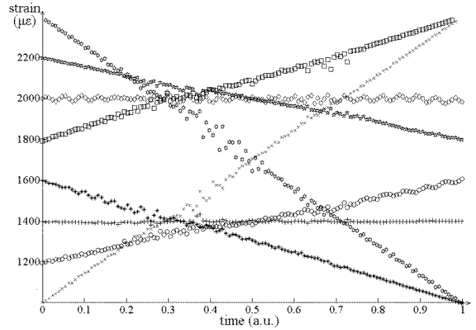
Fig. 7. Simulation results for densely multiplexed system.
