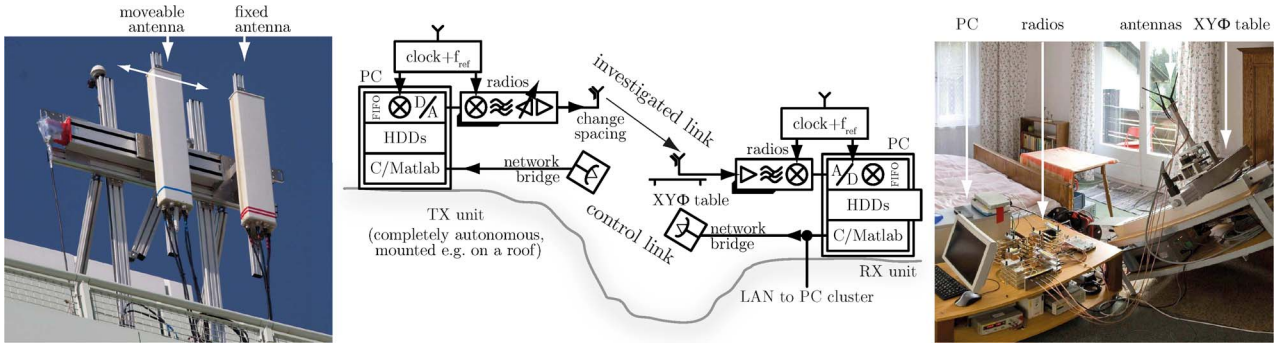
Fig. 7. The measurement testbed [35].
