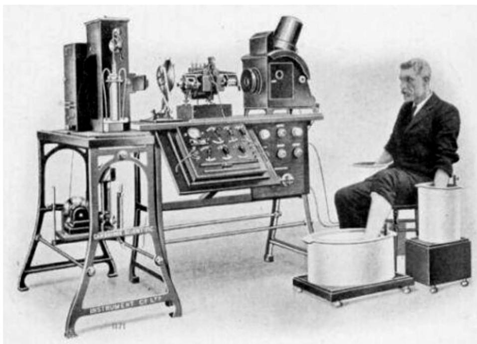
Fig. 5. Complete instrumentation for ECG. Courtesy of the University of Leiden, The Netherlands.
