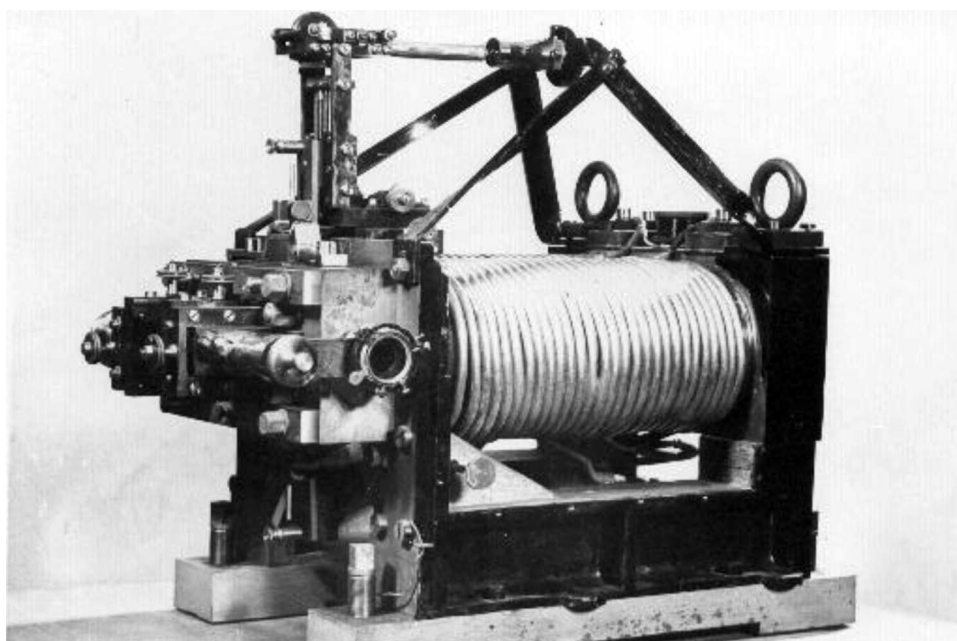
Fig. 3. String galvanometer of Einthoven, including cooled magnet, vertically mounted string, and an optical viewer. Courtesy of the University of Leiden, The Netherlands.
