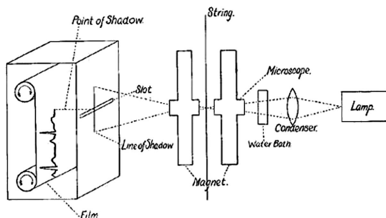
Fig. 2. Schematic diagram of string galvanometer of Einthoven for ECG. Courtesy of the University of Leiden, The Netherlands.
