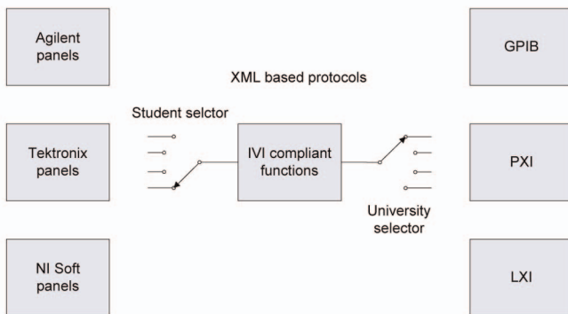
Fig. 9. Virtual front panel and hardware platform selections.
