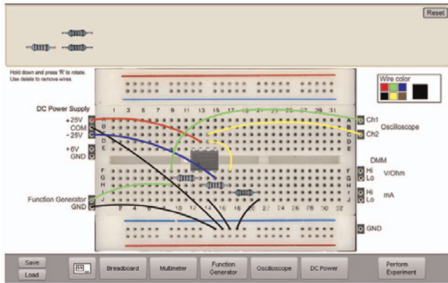
Fig. 3. Virtual breadboard.
