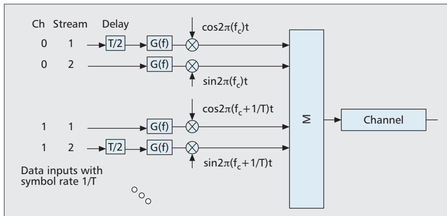
Figure 8. OFDM-OQAM implementation with staggered time-delayed subchannels (adapted from Saltzberg [9] and Hirosaki [11]). Only two transmitter subchannels are shown, with the pattern repeating for additional subchannel pairs and with a comparable structure in the receiver.
