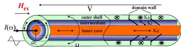
Fig. 1. Domain structure of amorphous wire. Circular domains exist in the outer region and the inner core has an axial magnetization. The driving ac current I(\omega) generates a circular magnetic field, response to which is characterized by the circumferential (transverse) permeability \mu . This response is highly sensitive to the applied magnetic field H_{ex} , and could be measured as a voltage V induced across the wire ends.
