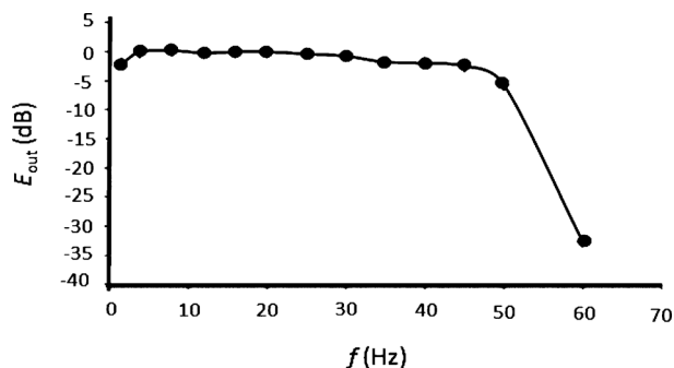
Fig. 10. Frequency characteristics of MI gradiometer for biomagnetic measurement.
