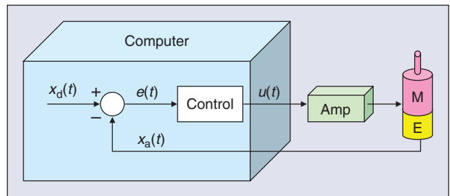
Figure 4. Computer control of a robot joint, showing the motor (M), encoder (E), and power amplifier (Amp).
